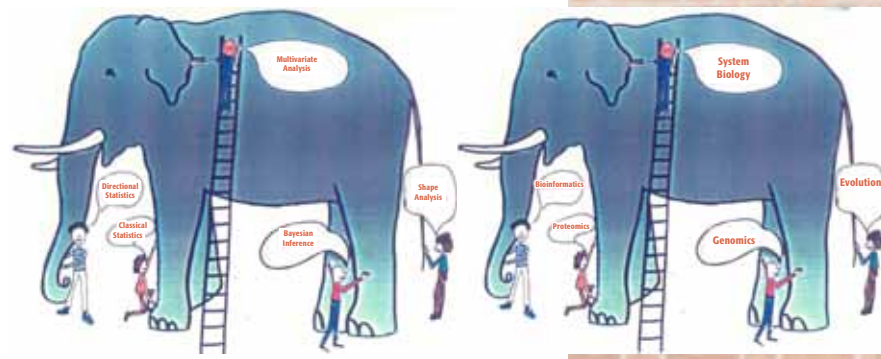
Holistic Statistics
